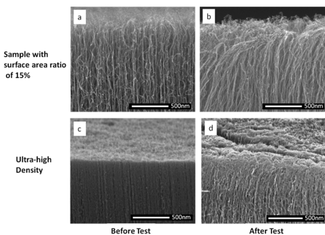
Figure 2. SEM images of the VACNTs (a and c) before and (b and d) after the adhesion tests. (a and b) Low-density VACNTs exhibit sufficient intertube space for the nanotubes to bend, resulting in a larger side-wall contact and increased adhesion, whereas (c and d) highly packed arrays have a very limited spacing for bending, resulting in a considerably reduced side-wall contact and consequently no adhesion at all.
