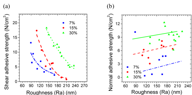
Figure 3. Dependence of (a) shear and (b) normal adhesion strength on the surface roughness of the VACNT samples; 7, 15, and 30% indicate the packing density of the arrays.
